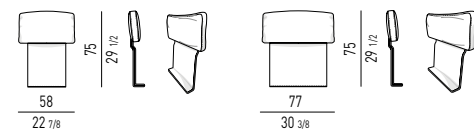
POGGIATESTA OPTIONAL "FREEMAN DUVET" "FREEMAN DUVET" OPTIONAL HEADRESTS
