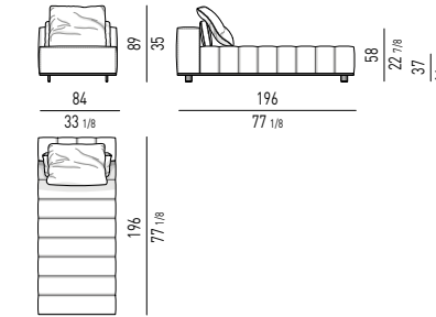
COUCH CM 84X196
