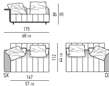
ELEMENTO TERMINALE CM 175 ELEMENT WITH 1 ARMREST CM 175
