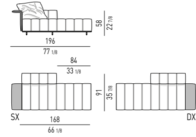
ELEMENTO TERMINALE PENISOLA CM 196 - SCHIENALE CM 84 OPEN-END ELEMENT WITH 1 ARMREST CM 196 - BACKREST CM 84
